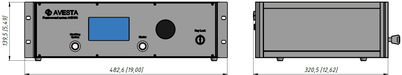
ANTAUS-10W-4u/2.5M laser head and control unit in mm
